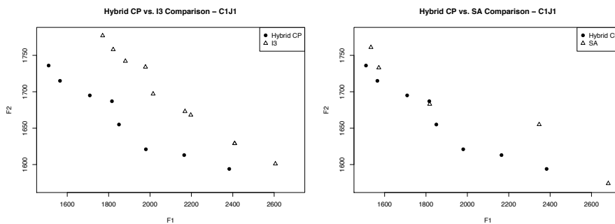
Figure 3. Hybrid CP-based methodology vs. using only the I3 heuristic (left) or another state-of-the-art approach for the VRPTW (right)
