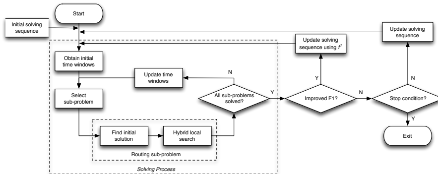
Figure 2. Flow diagram for the Sequence Iterative Method (SIM)
